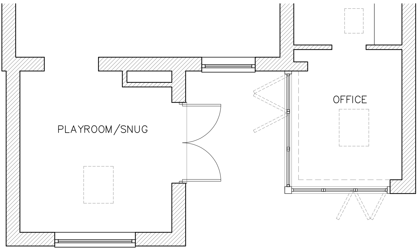
Ground Floor Plan As Existing
