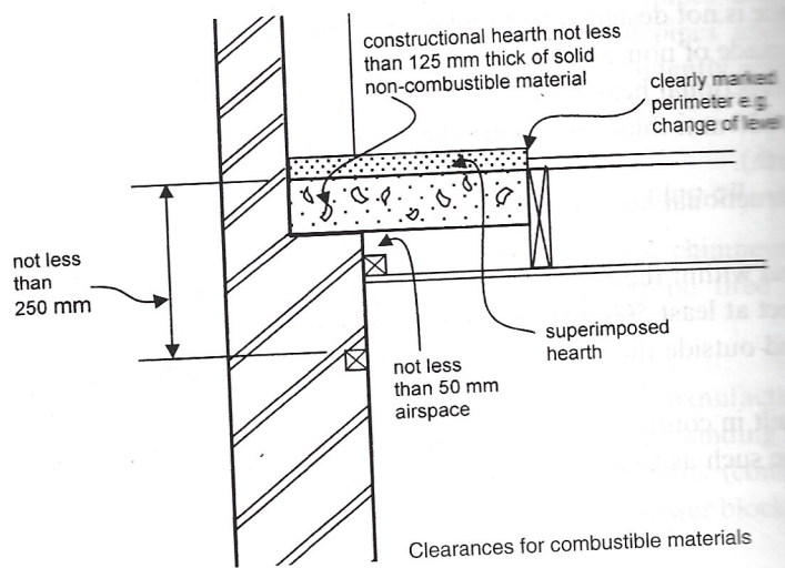
Fig. 14.11 Hearths for appliances burning solid fuel.
