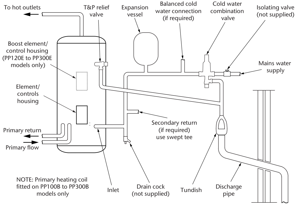
Fig 6 - Typical installation - schematic
